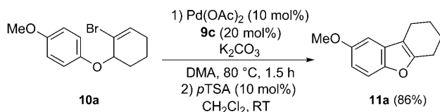
Scheme 2. Optimized benzofuran formation. DMA = N,N -dimethylacetamide, pTSA = toluene- p -sulfonic acid.
